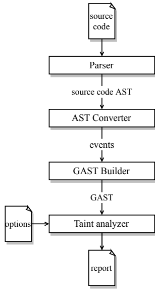
Fig. 1. The GT tool data flow and architecture
